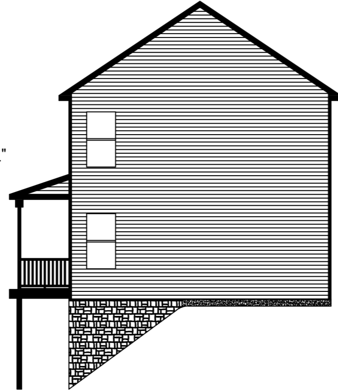
Elevation - Left
