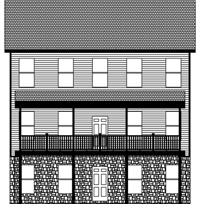
Elevation - Rear
